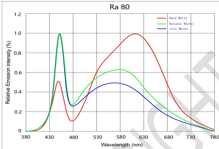
Fig.1-Spectrum Distribution
