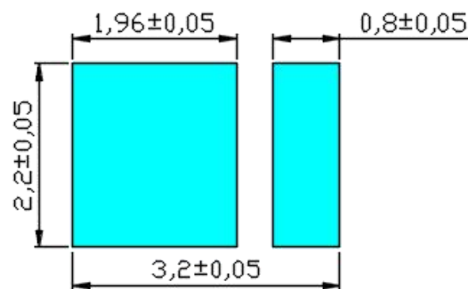
Recommended PCB solder PAD
