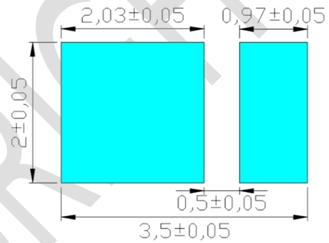
Recommended PCB solder PAD
