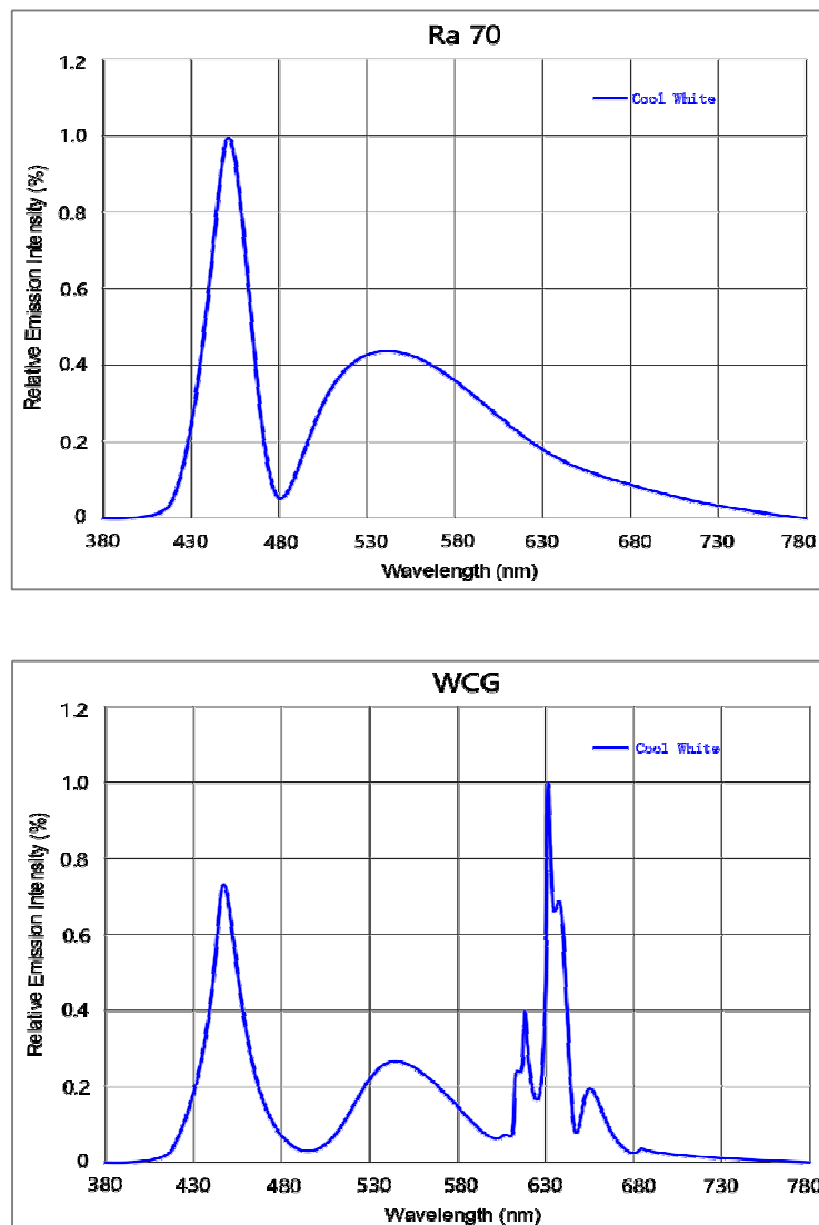
Fig.1-Spectrum Distribution
