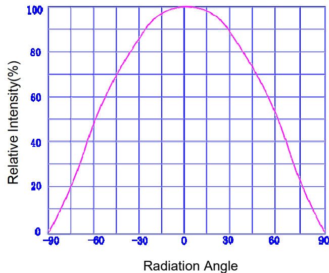
Fig.7- Directivity
