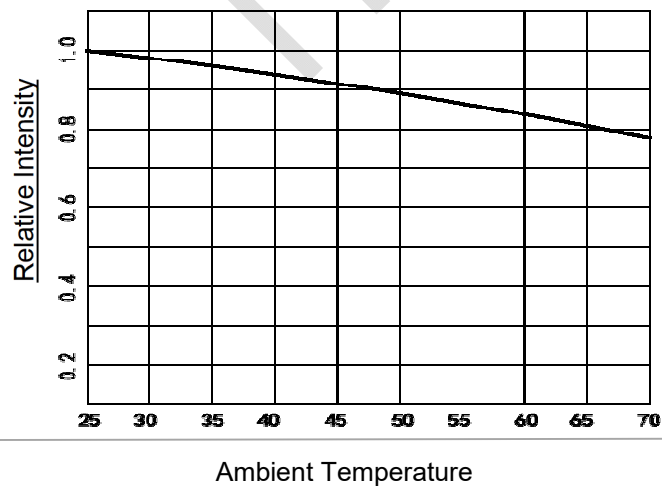
Fig.5- Relative Intensity vs. Ambient Temp.
