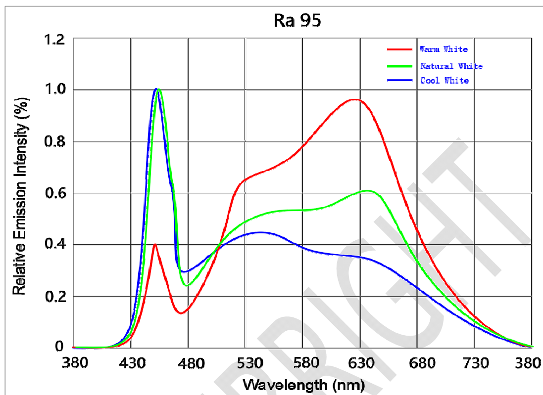
Fig.1-Spectrum Distribution
